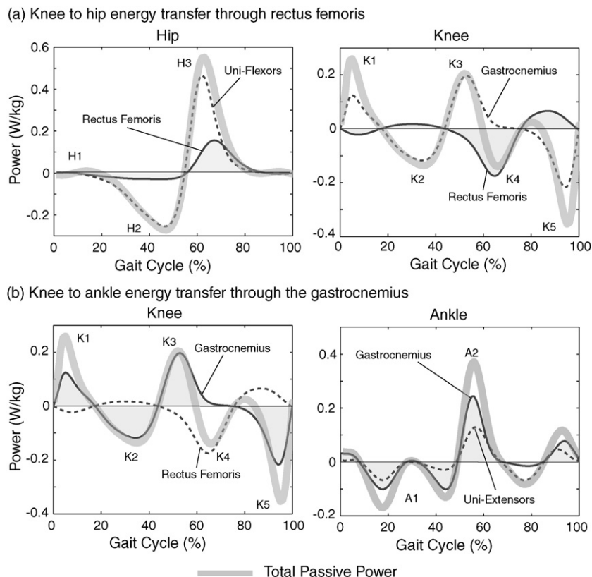
Fig. 5. Shaded regions of the power curves represent the energy absorbed and released at the specific joints via the biarticular rectus femoris and gastrocnemius. (a) Energy absorption at the knee in the rectus femoris occurs coincidentally with energy release at the hip, suggesting that the muscle is facilitating simultaneous energy transfer across joints. (b) In contrast, energy transfer between the knee and ankle displays more of a stretch-recoil effect in which the gastrocnemius stores energy as the knee extends (K2) and releases that energy later when the knee flexes (K3) and ankle plantarflexes (A2).
