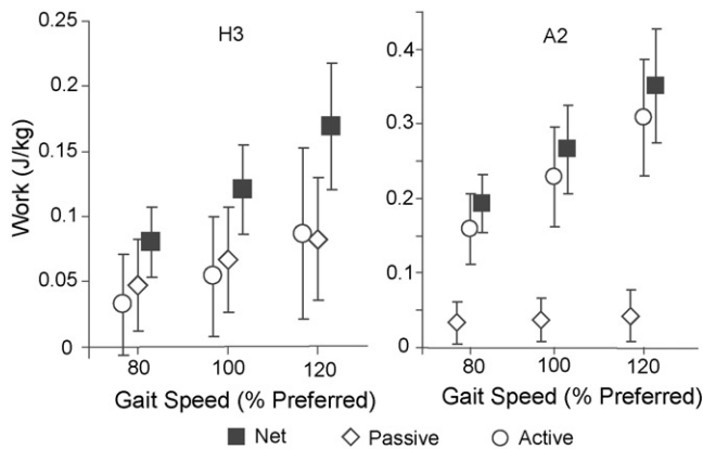
Fig. 3. Speed effects on passive, active, and net works during hip flexor (H3) and ankle plantarflexor (A2) power bursts. Passive work, attributed to stretch of soft tissues, increased significantly ( p < 0.05 ) with speed for both the hip and ankle.
