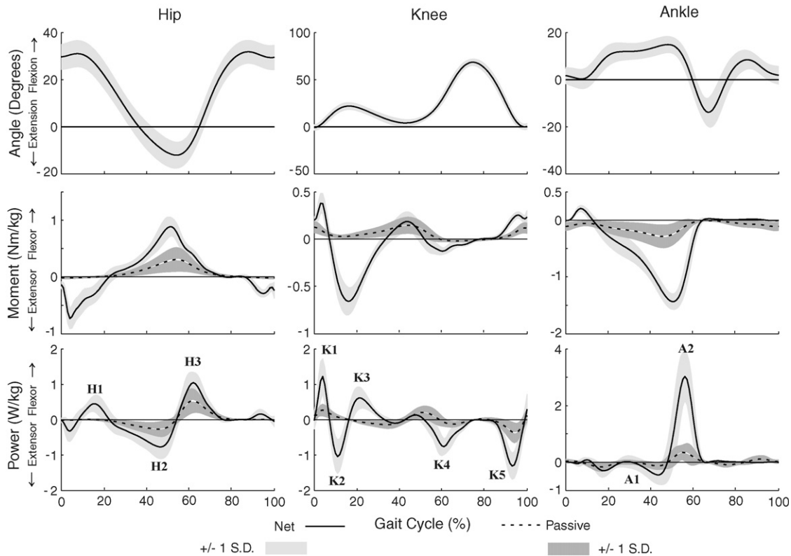
Fig. 2. Ensemble-averaged joint angle, net joint moment, and net joint power curves from gait analysis for 20 subjects. Overlaid are the average ( \pm 1 S.D.) estimated passive joint moment and joint power curves. The largest passive moments arise in hip flexion between 30% and 60% of the gait cycle, contributing substantially to both the H2 and H3 power bursts.
