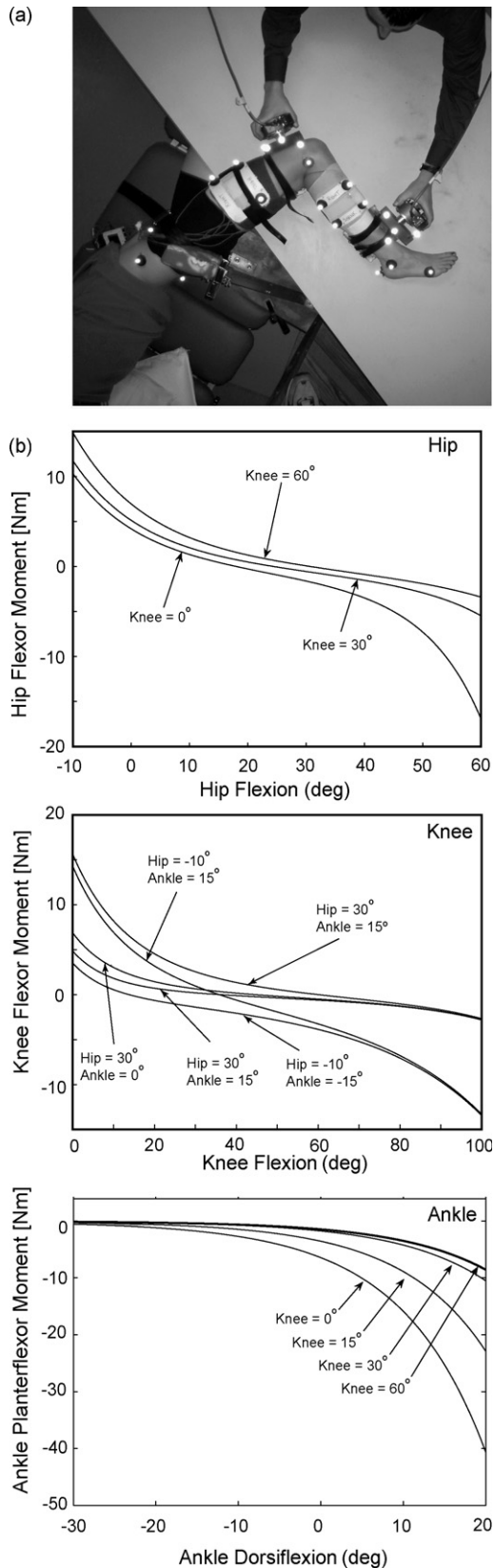
Fig. 1. (a) During passive testing, the subject was in a side lying position with the pelvis restrained while the dominant limb was manipulated using two 3D handheld load cells. The image reflects a top view of the set-up with the table angled posterior to the subject to allow for full hip extension and
