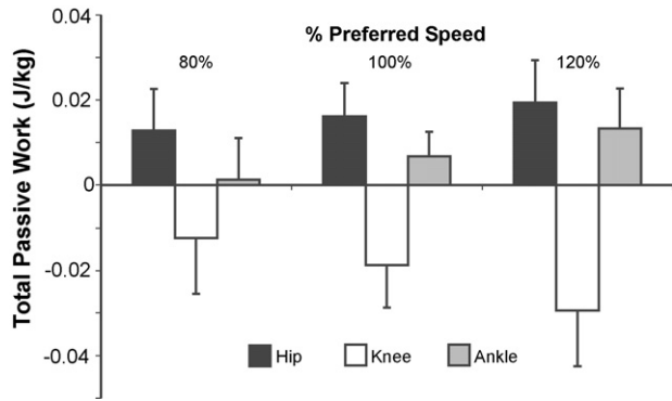
Fig. 4. The total passive work at an individual joint across a gait cycle can be non-zero due to biarticular muscle stretch transferring energy across joints. At all speeds, a significant amount of energy was absorbed at the knee ( p < 0.05 ). This energy was returned at the hip (all speeds) and ankle (100%, 120%) via rectus femoris and gastrocnemius stretch, respectively.
